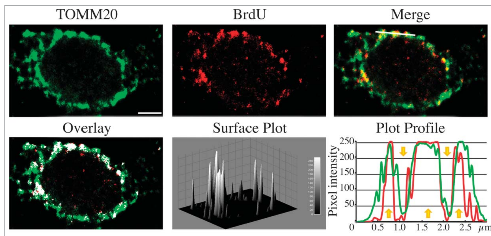
Figure 25. Confocal microscopy deconvolved (AutoQuant X3) images and colocalization image analysis (ImageJ 1.47; Imaaris 7.6) through a local approach showing perinuclear mitochondrial biogenesis in hippocampal neuronal cultures. The upper channels show TOMM20 (green channel), BrdU (for visualization of newly synthesized mitochondrial DNA, red channel), and merged fluorescence channels. Overlay, corresponds to the spatial pattern of software thresholded colocalized structures (white spots) layered on the merged fluorescence channels. Surface Plot, or luminance intensity height, is proportional to the colocalization strength of the colocalized structures (white spots). Plot Profile, corresponds to the spatial intensity profiles of the fluorescence channels of the white line positioned in the Merge image. Yellow arrows indicate a qualitative evaluation of the spatial association trends for the fluorescence intensities. Arrows pointing up indicate an increase in the colocalization, while arrows pointing down show a decrease. Scale bar: 2 \mu\text{m} . This figure was modified from previously published data 2187 and provided by F. Florenzano.
